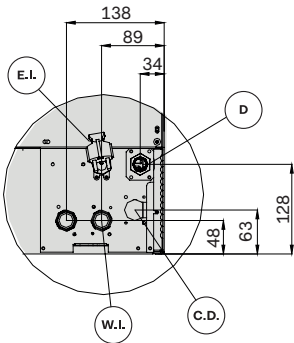
Rear view (Water and electrical connections)
